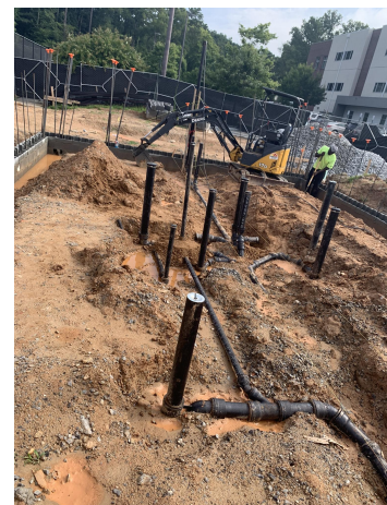
CSK- Concession Plumbing Underground Rough-In
